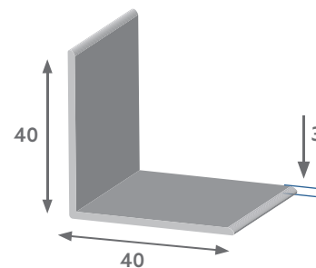
R 4022 | Cantoneira 40x40x3mm
