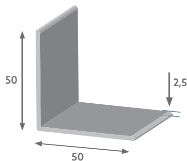
R 4068 | Cantoneira 50x50x2,5mm
